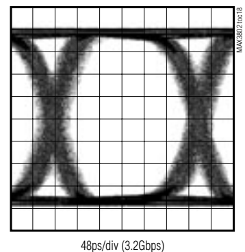
EQUALIZER OUTPUT EYE DIAGRAM AFTER 72ft OF 75Ω RG179 CABLE (300mVp-p SINGLE ENDED, 2^{23} - 1 PRBS)
